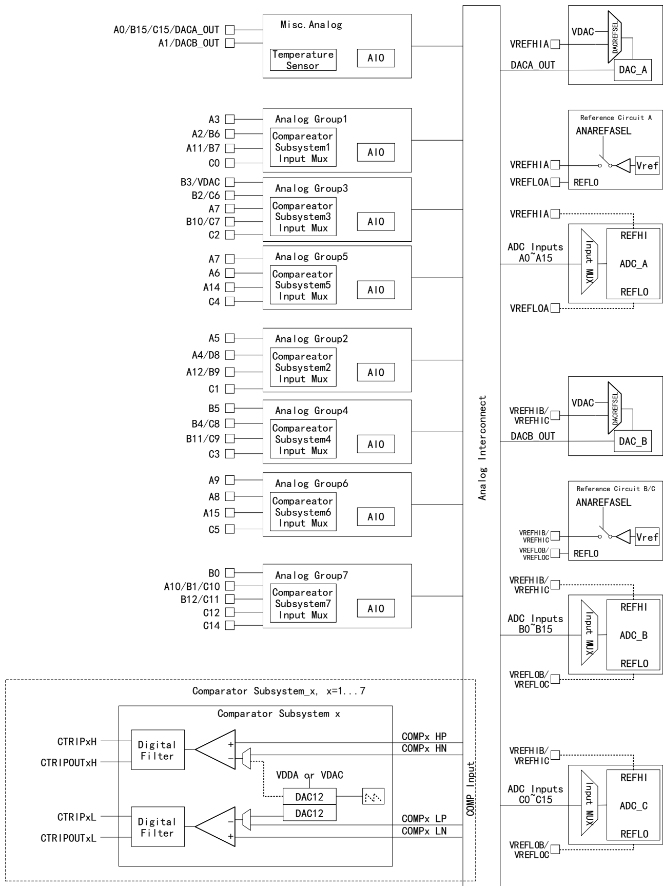
Figure 37 Analog Subsystem Block Diagram (100-pin)
