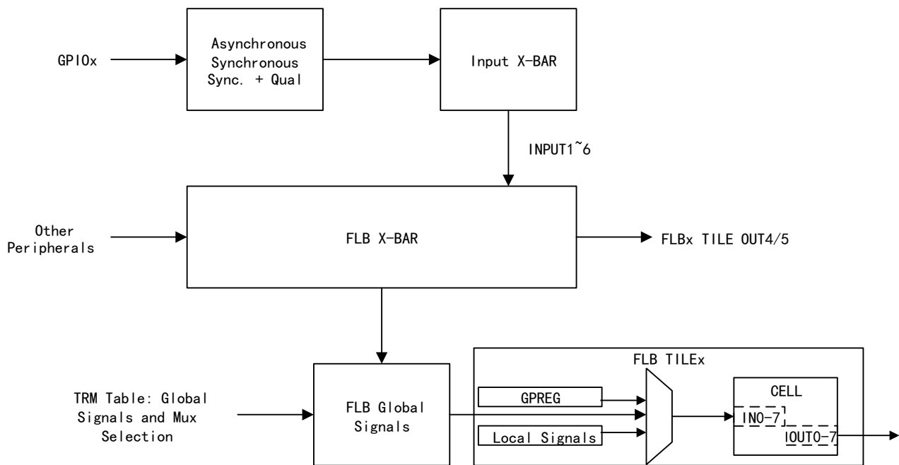
Figure 11 TILE Connection from GPIO to FLB
