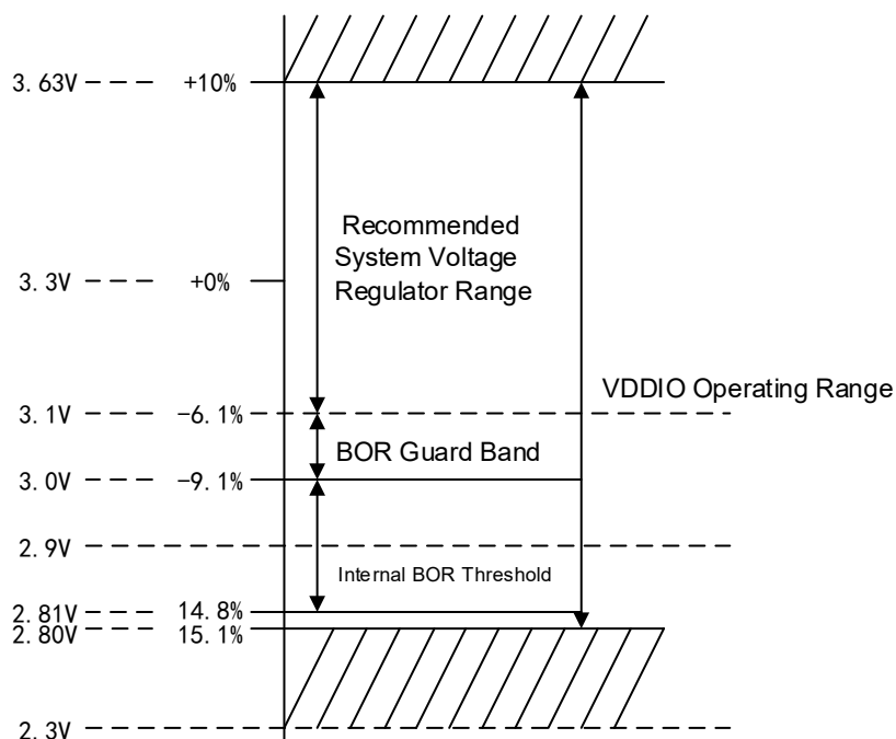
Figure 12 Supply Voltage
