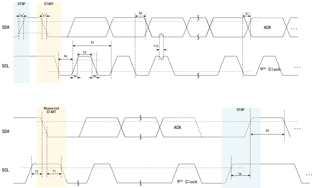
Figure 70 I2C Timing Diagram
