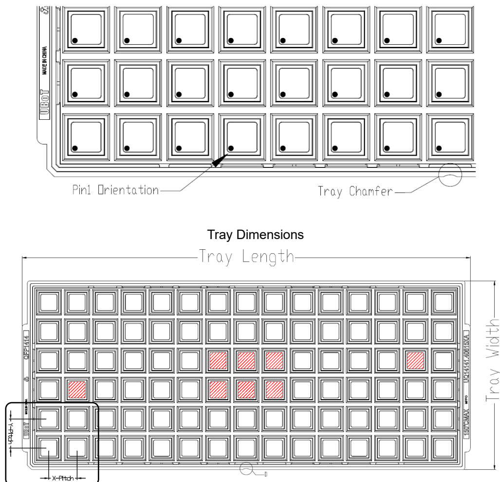
Figure 96 Tray Packaging Diagram
