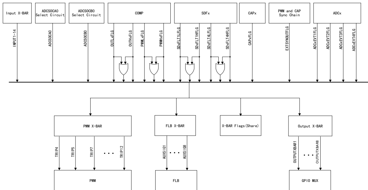
Figure 6 Output X-BAR and PWM X-BAR Sources
