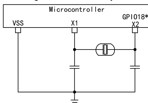
Figure 22 External Crystal
