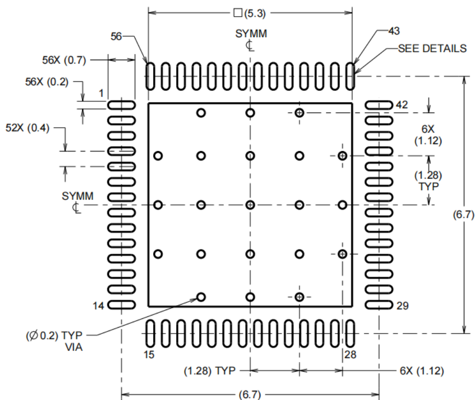
Figure 94 QFN56, 7x7mm Welding Recommendations
