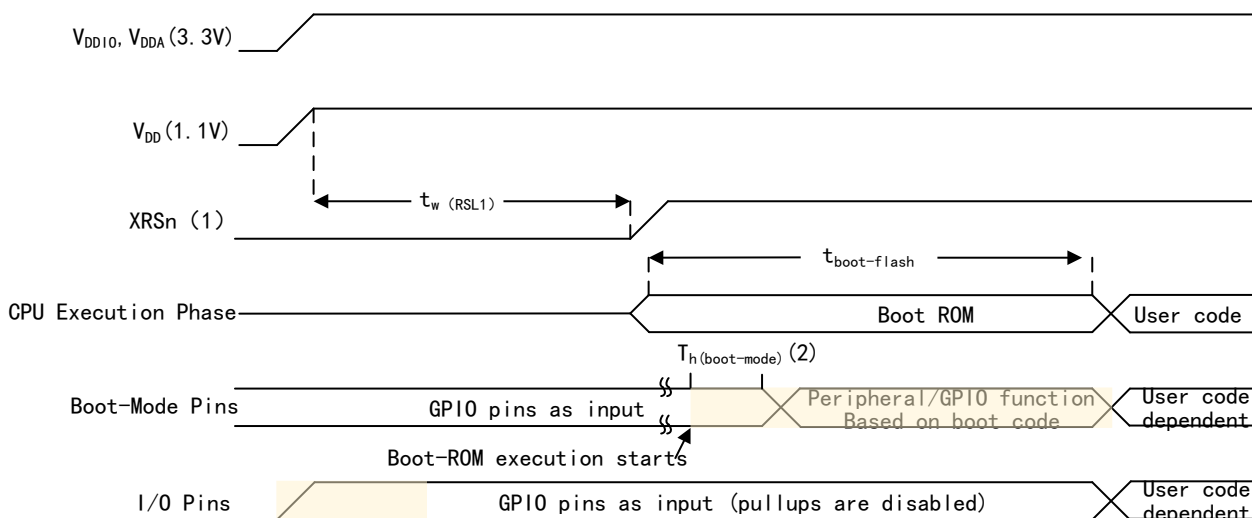
Figure 17 Power-on Reset
