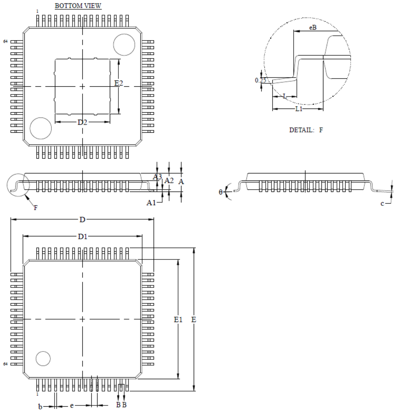
Figure 92 E-LQFP64 Package Diagram
