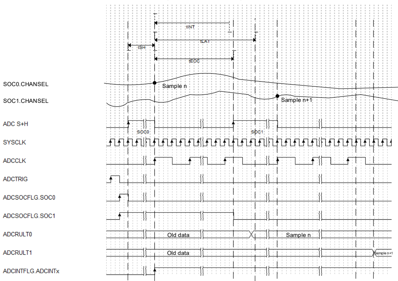
Figure 45 ADC Timing
