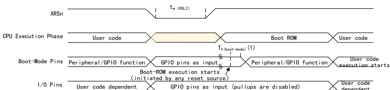
Figure 18 Hot Reset
