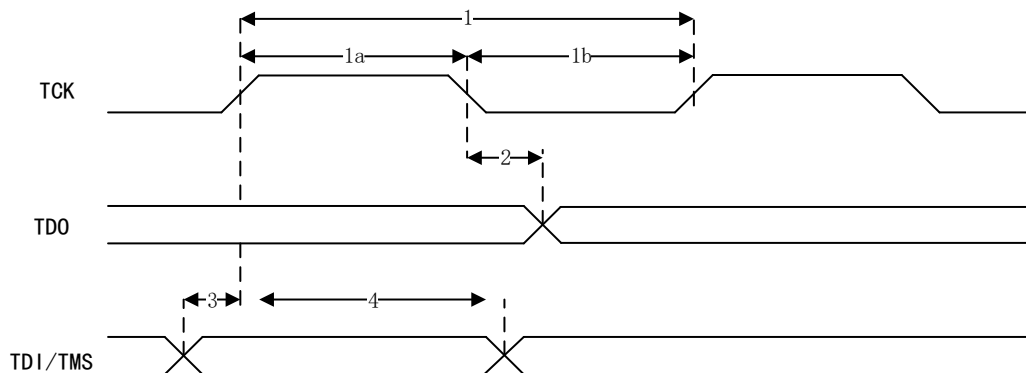
Figure 28 JTAG Timing
