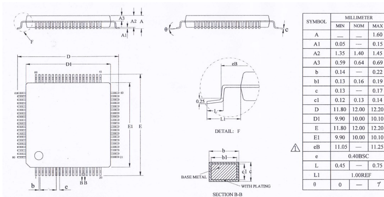
Figure 89 LQFP80 (10mm*10mm) package information
