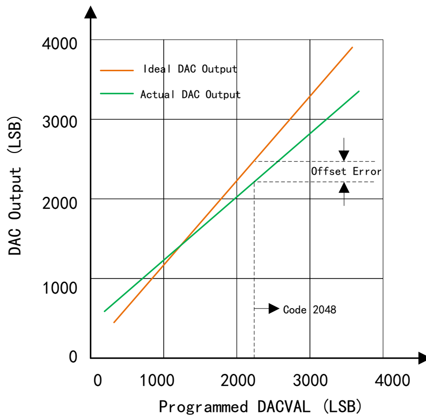
Figure 47 Offset of Buffer DAC
