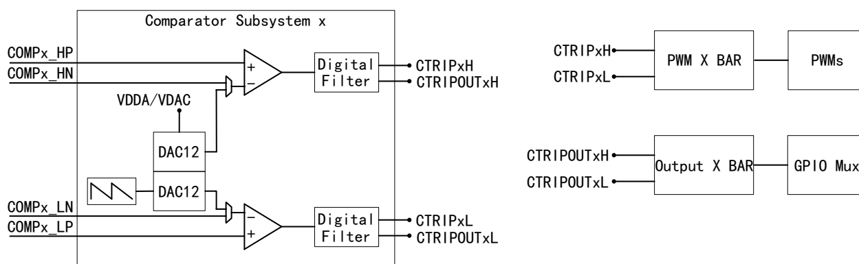
Figure 50 COMP Connection
