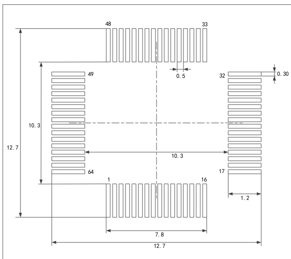
Figure 91 LQFP64, 10x10 Welding Layout Recommendations
