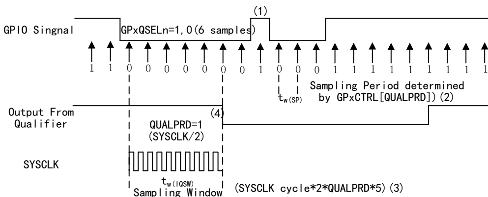
Figure 31 Sampling Mode
