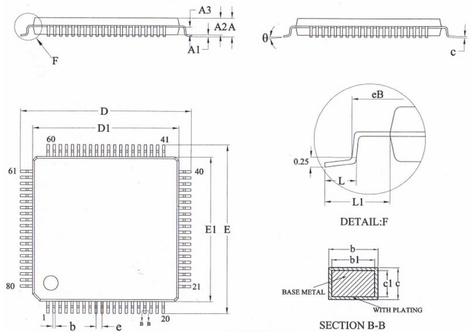
Figure 87 LQFP80 Package Diagram
