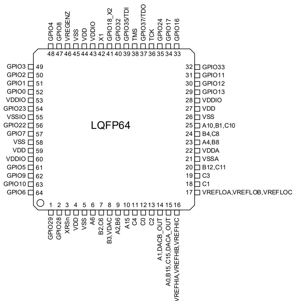
Figure 3 G32R5xx Series LQFP64/E- LQFP64 Pin Distribution Diagram
