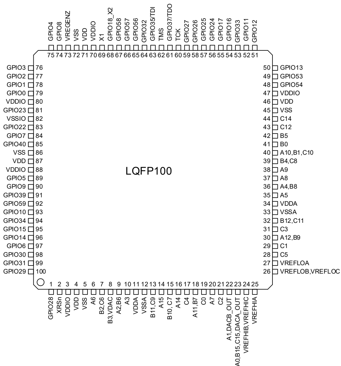
Figure 1 G32R5xx Series LQFP100/E- LQFP100 Pin Distribution Diagram
