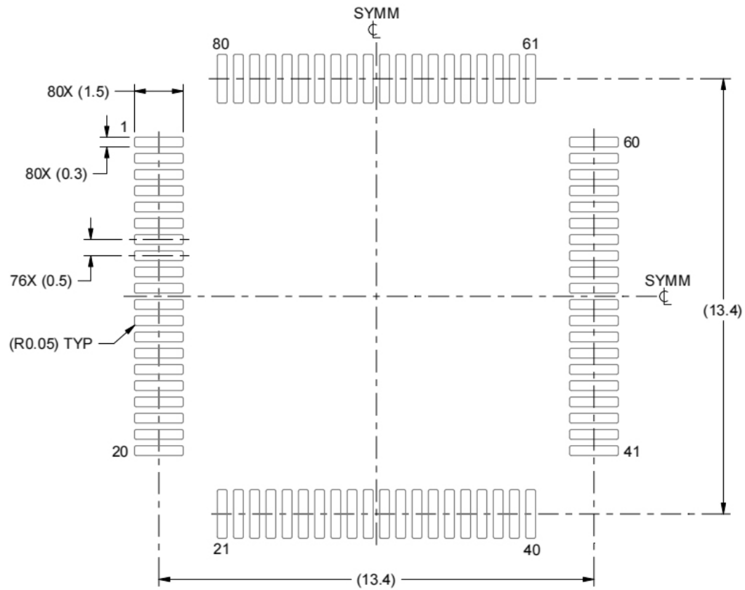
Figure 88 LQFP80, 12x12mm Welding Layout Recommendations
