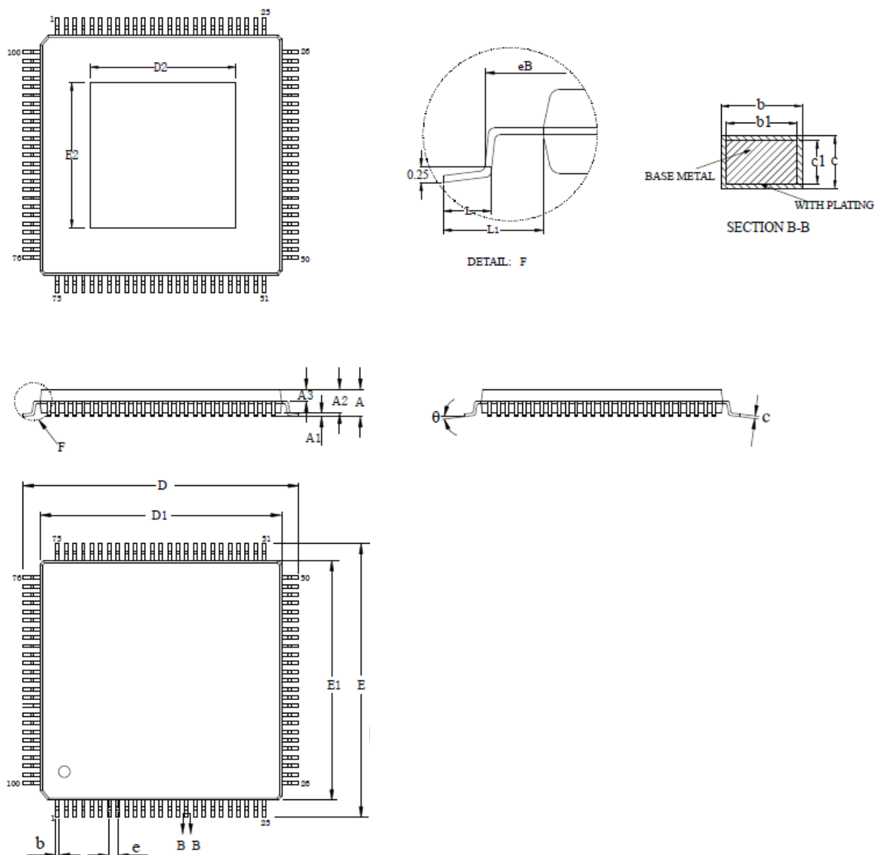
Figure 86 E-LQFP100 Package Diagram
