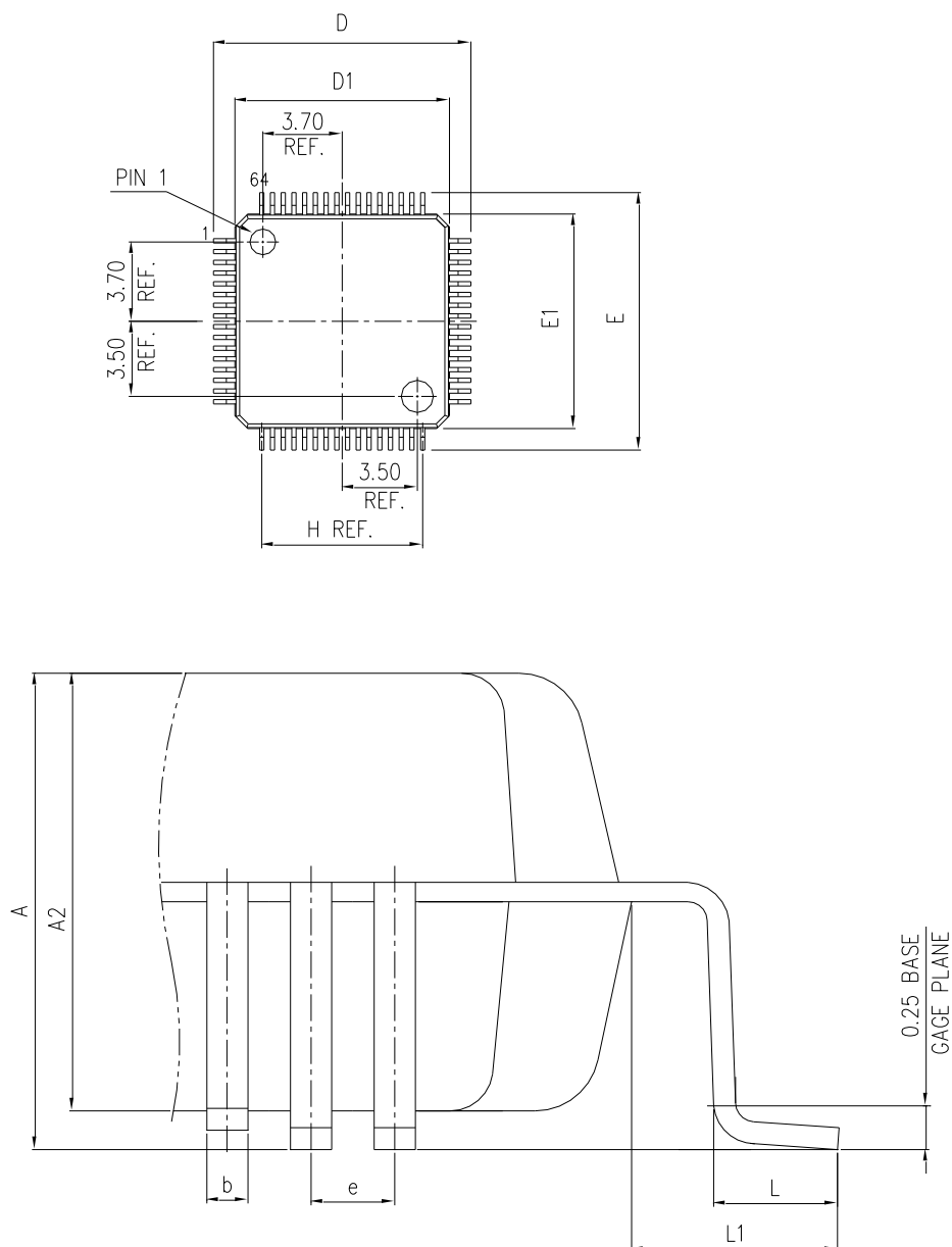
Figure 90 LQFP64 Package Diagram
