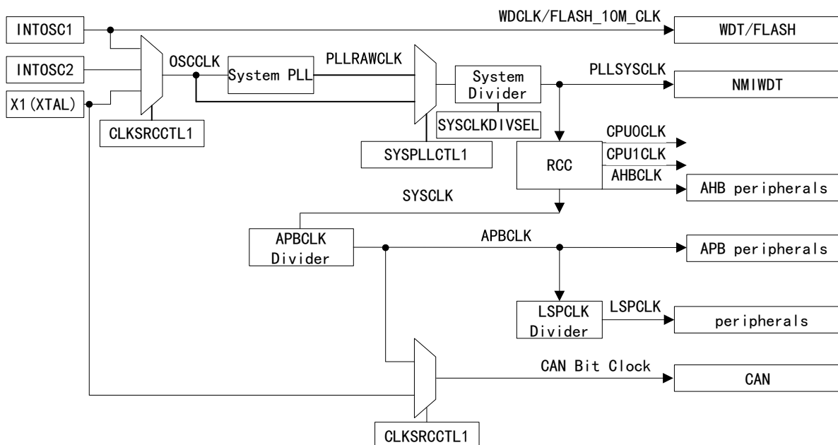
Figure 19 Clock Source
