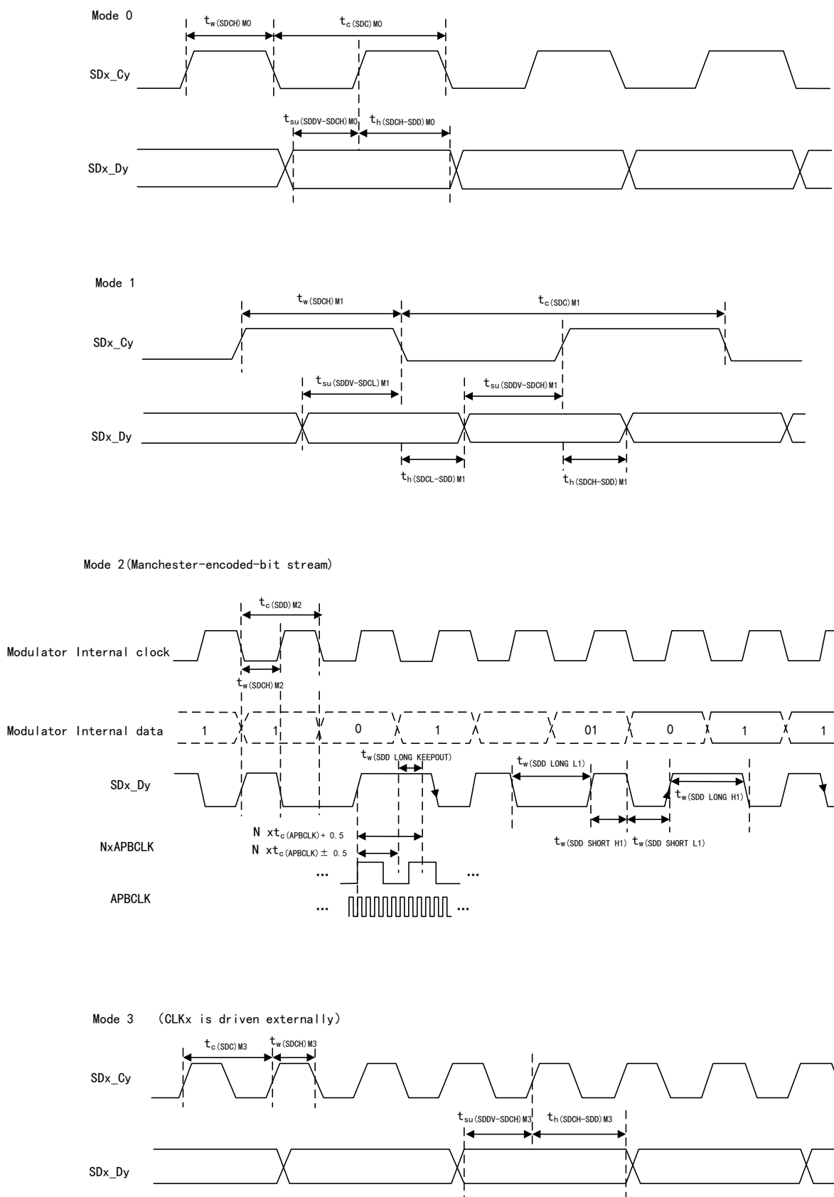
Figure 67 SDF Timing Diagram
