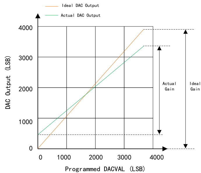
Figure 54 Static Gain of COMP DAC
